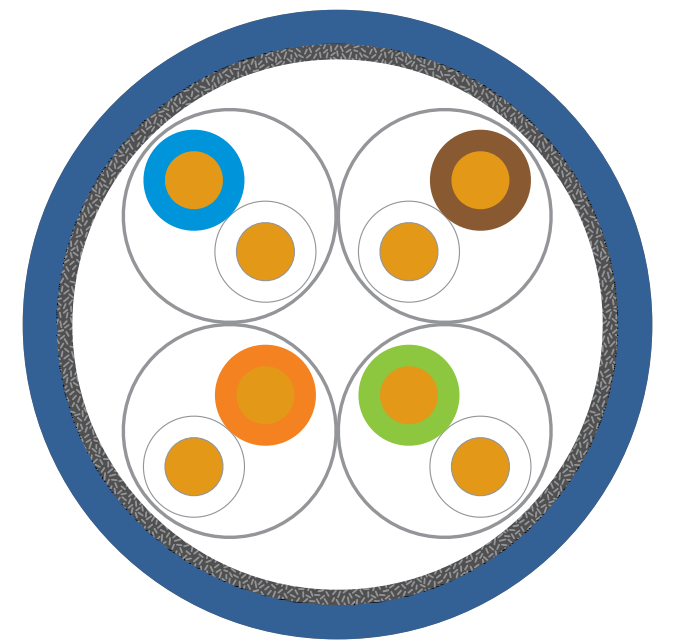
S/FTP
