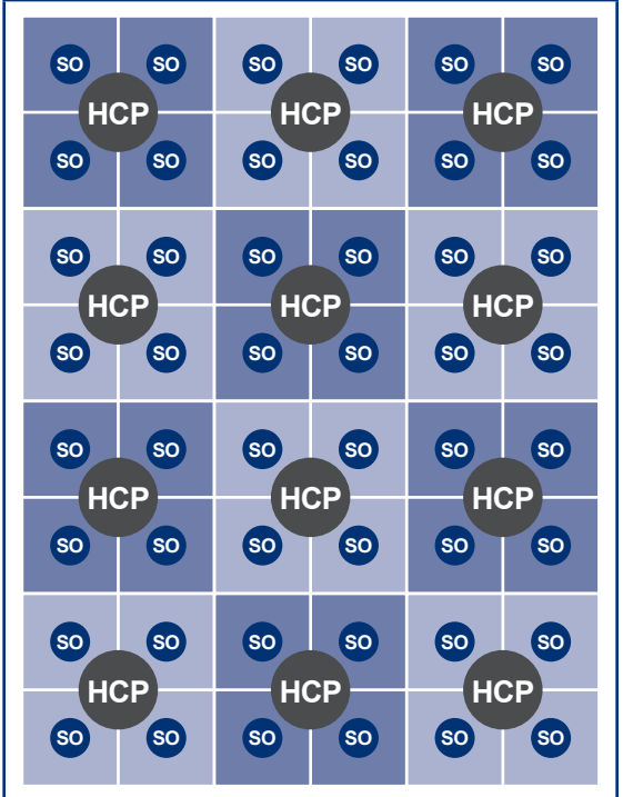
Grid pattern of HCPs positioned to support for Service Outlet coverage
